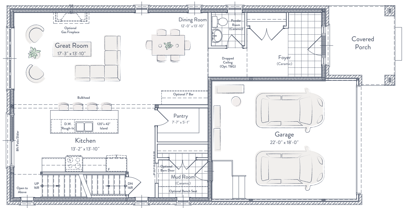
MAIN LEVEL: 1114 SQ FT
